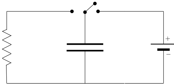
FIG. 3: A circuit diagram of our experiment. The double switch allows the capacitor to be charged up from an emf source and then to discharge through a resistor which heats up, thereby serving as a measuring device for the electrostatic energy that had been stored.
